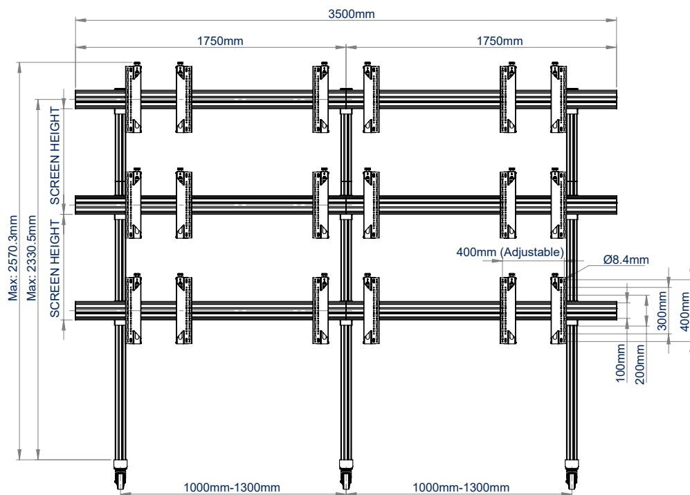
FRONT VIEW
