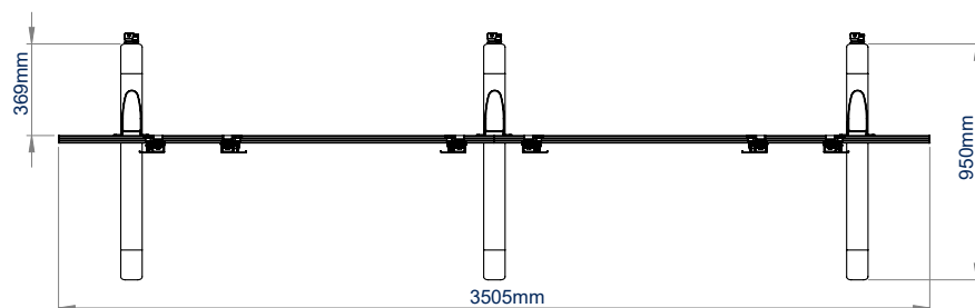
TOP VIEW
